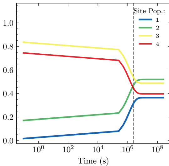
Time Evolution of Site Populations under \mathcal{L} , \mathcal{L}_{\text{eff}} , and \mathcal{L}_{\text{eff}}^{\text{red}} N=4 ; N_{\text{dimers}}=2 ; N_{\epsilon}=0 ; J = 10^{-1} ; \epsilon = 10^{-4} ; seed=902
